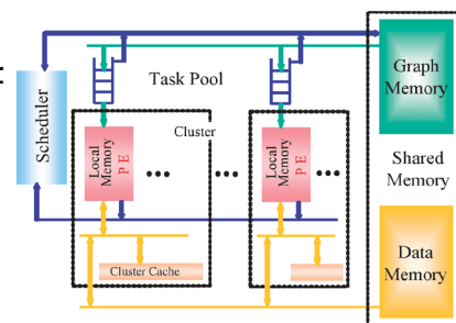
Fig1. Clustered Parallel Reduction System
