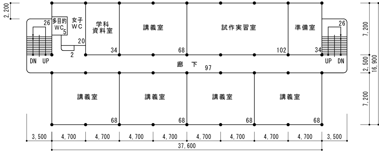
8号棟3階平面図（改修前）S=1/300
