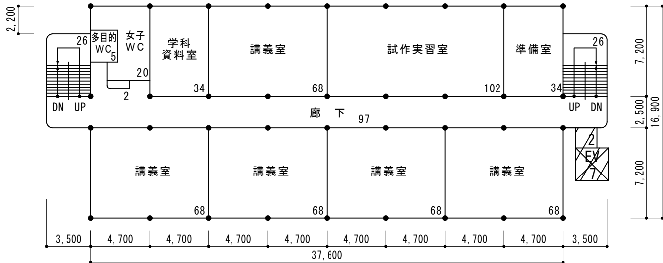
8号棟3階平面図（改修後）S=1/300
