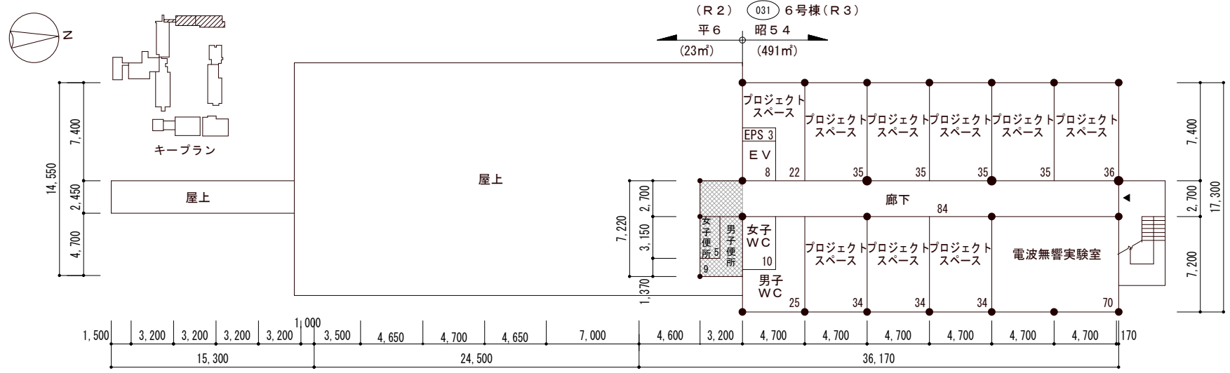
6号棟3階改修後平面図 (491 m 2 ) S=1/400
